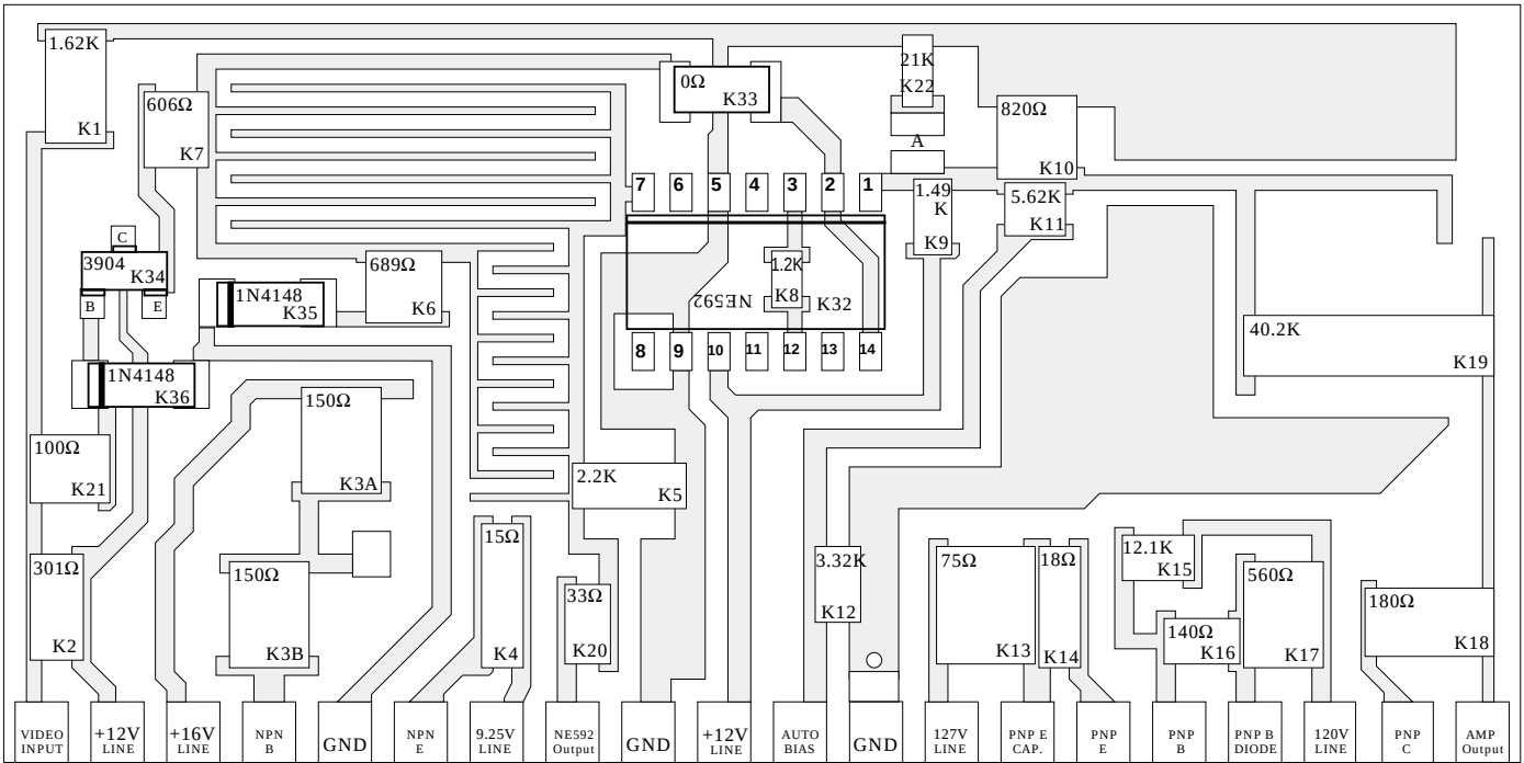
Video Amplifier Resistor Array "K Film" K P/N CPR0510
