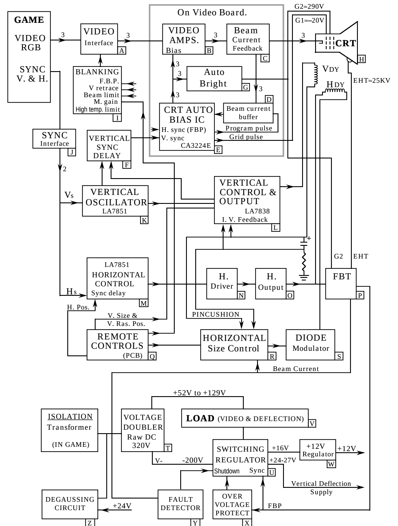
XX93 Monitor Block Diagram.
